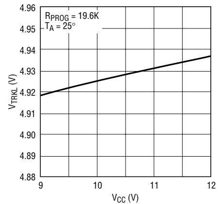
Trickle Charge Threshold Voltage vs V_{CC}
