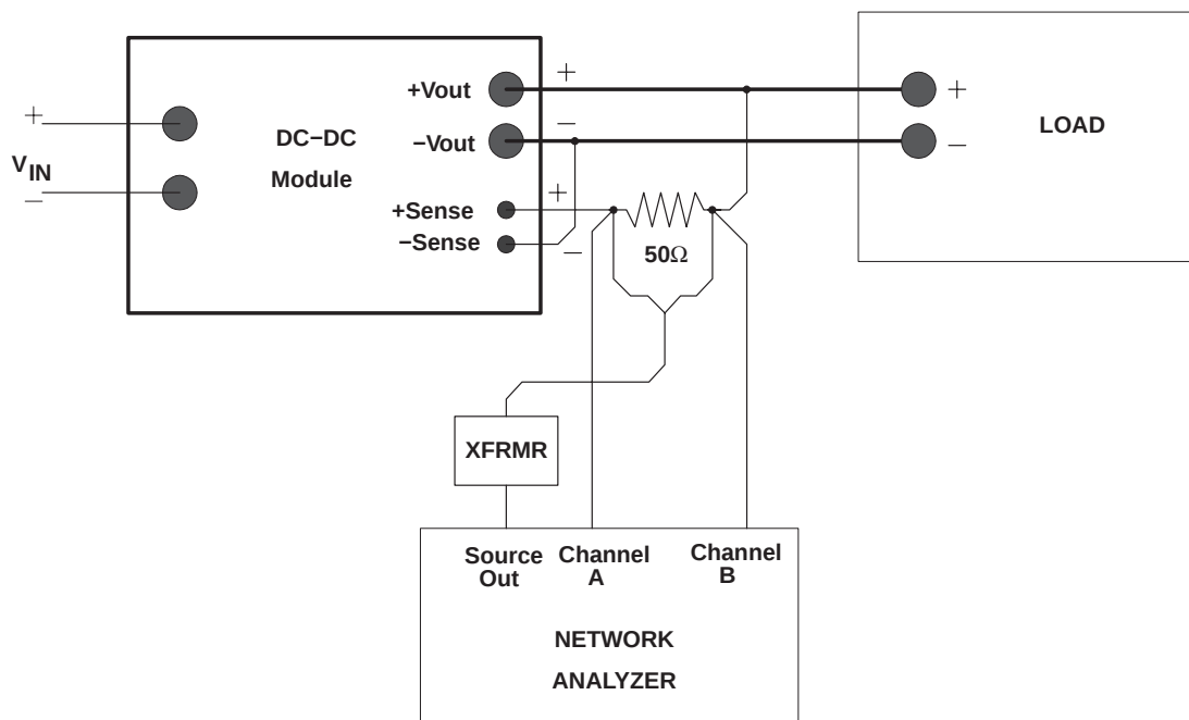
Figure 2. Measuring the Unity Gain Crossover Frequency
