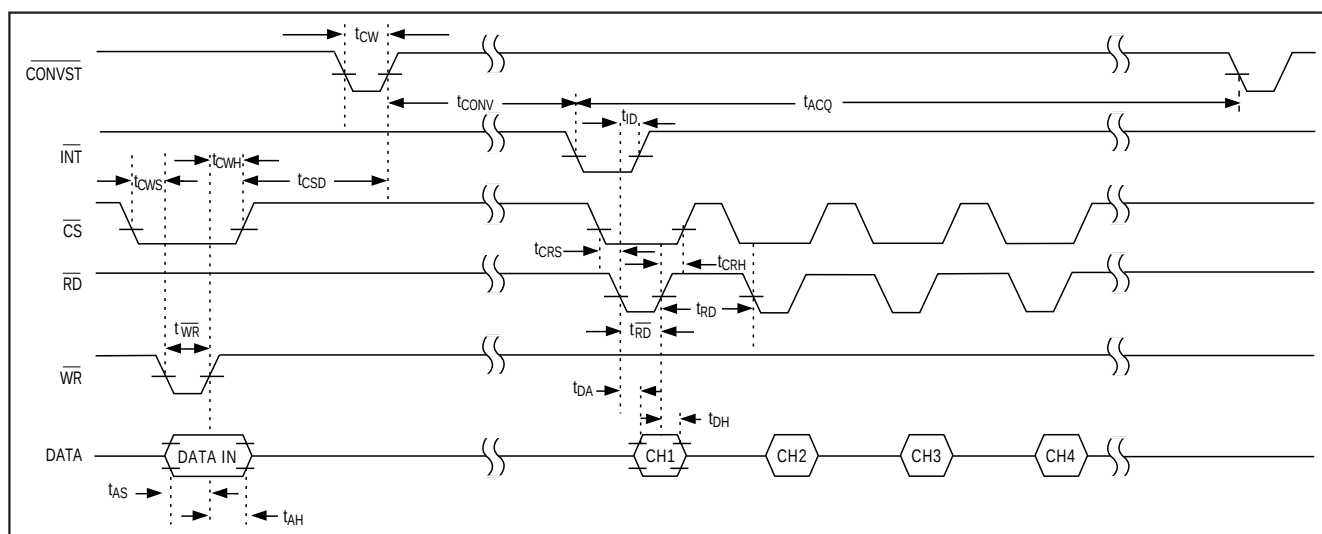
Figure 4. Timing Diagram
