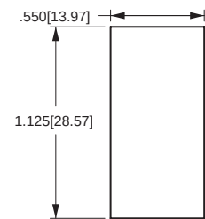
MOUNTING HOLE Panel Thickness: .020[.508] min. to .250[6.35] max.
