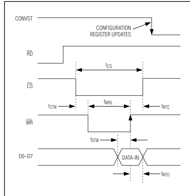
Figure 6. Write Timing
