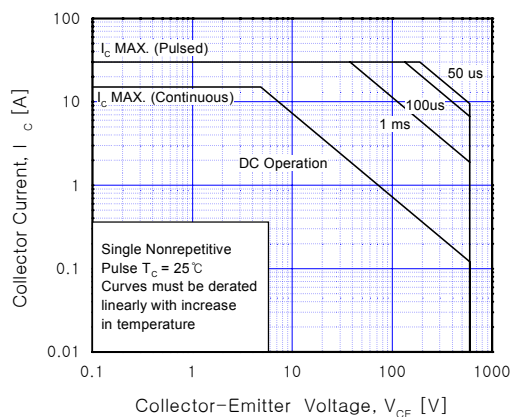
Figure 15. SOA Characteristics
