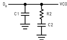
Figure 27. Passive Loop Filter
