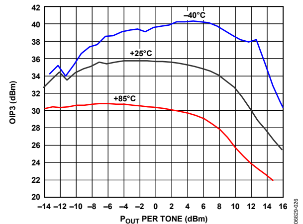
Figure 26. OIP3 vs. Output Power ( P_{OUT} ) and Temperature
