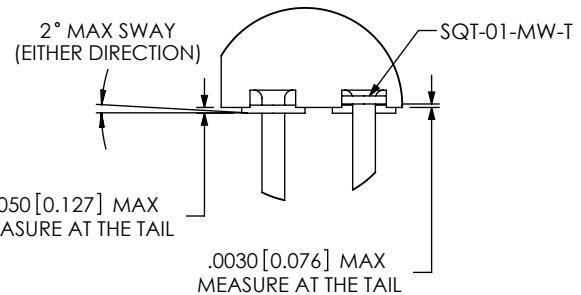
DETAIL 'B' SCALE 6:1
