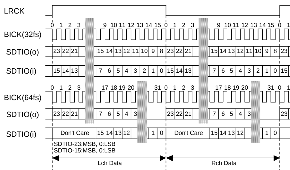
Figure 6. Mode 0 Timing
