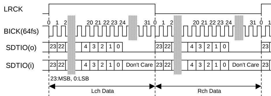
Figure 7. Mode 1 Timing
