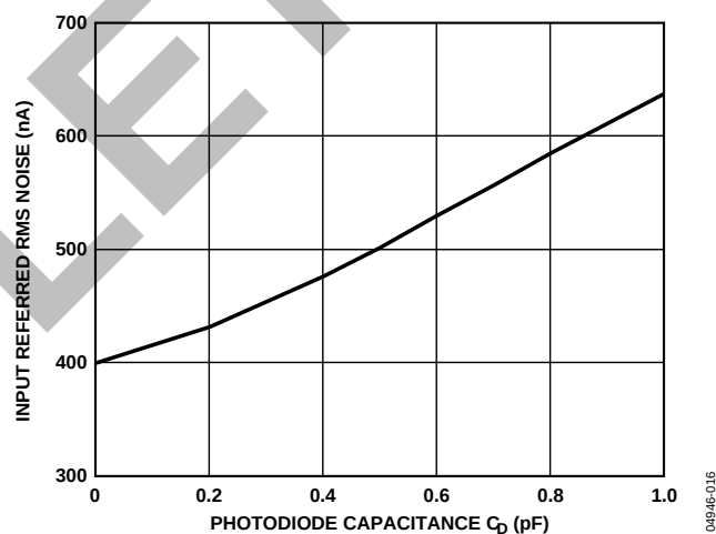
Figure 13. Input Referred Noise (DC to 4.0 GHz) vs. PD Capacitance
