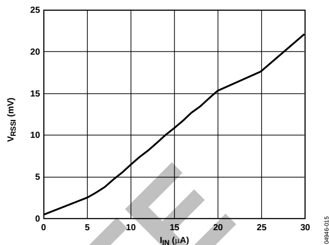
Figure 12. RSSI Voltage Output vs. Input Current (0 \mu A to 30 \mu A )
