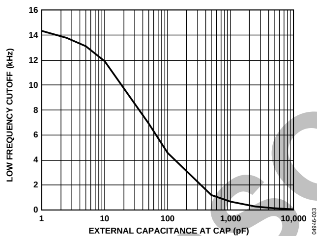
Figure 10. Low Frequency Cutoff vs. External Capacitance at CAP
