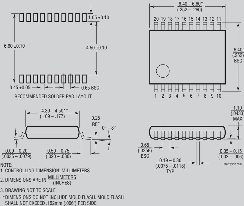
F Package 20-Lead Plastic TSSOP (4.4mm) (LTC DWG # 05-08-1650)
