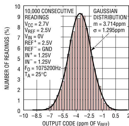
Noise Histogram (Output Rate = 52.5Hz, V_{CC} = 2.7V , V_{REF} = 2.5V )
