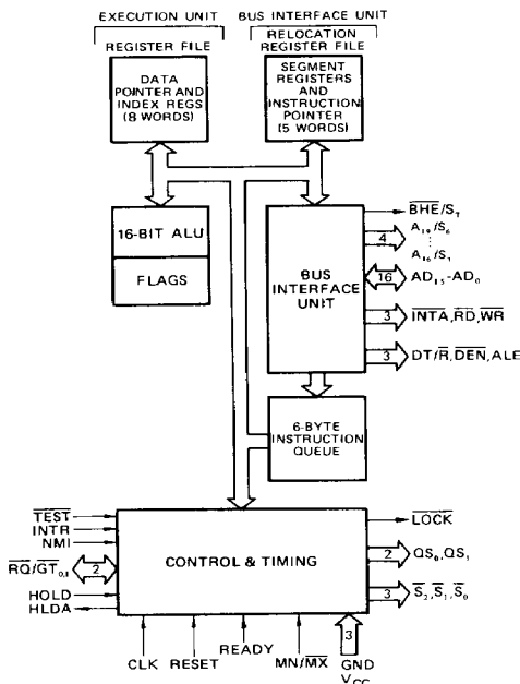
Fig. 1 - BLOCK DIAGRAM
