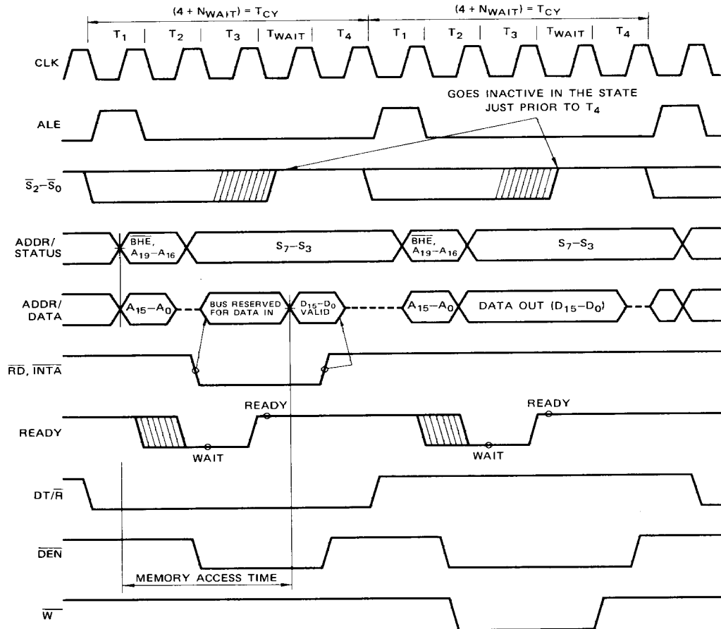
Fig. 5 - BASIC SYSTEM TIMING
