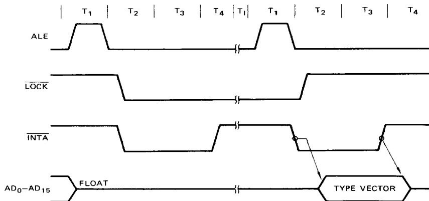
Fig. 6 — INTERRUPT ACKNOWLEDGE SEQUENCE
