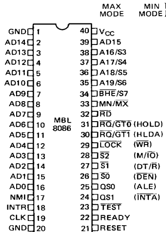
Fig. 2 - PIN CONFIGURATIONS
