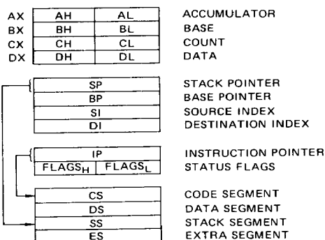
Fig. 7 — MBL 8086 REGISTER MODEL
