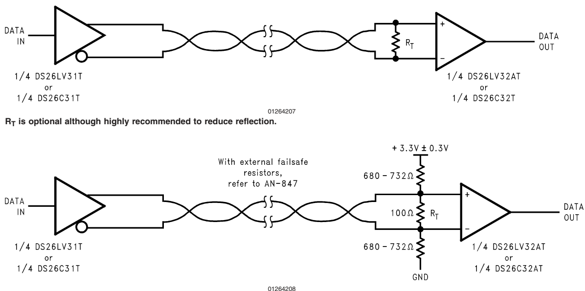
FIGURE 6. Typical Driver Connection
