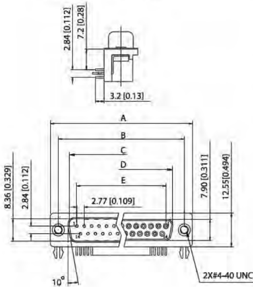
7.2mm[0.28"] Footprint
