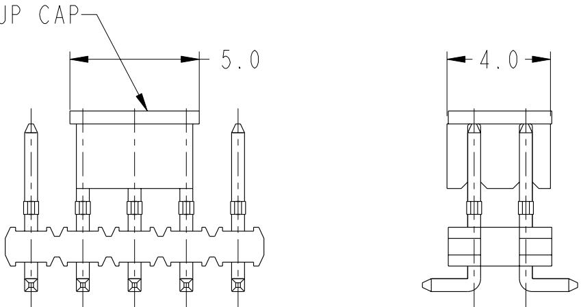
FIG. 1 NOTE 7 (c) SCALE 5:1
