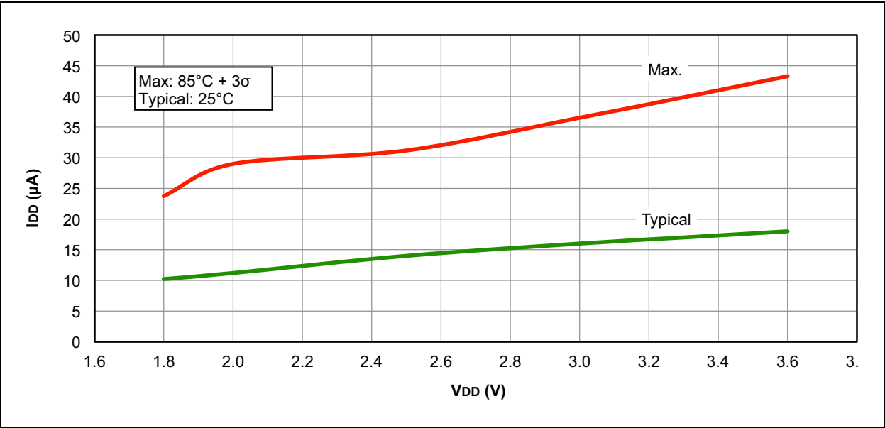
FIGURE 22-2: I DD , EC OSCILLATOR, LOW-POWER MODE, F osc = 500 kHz
