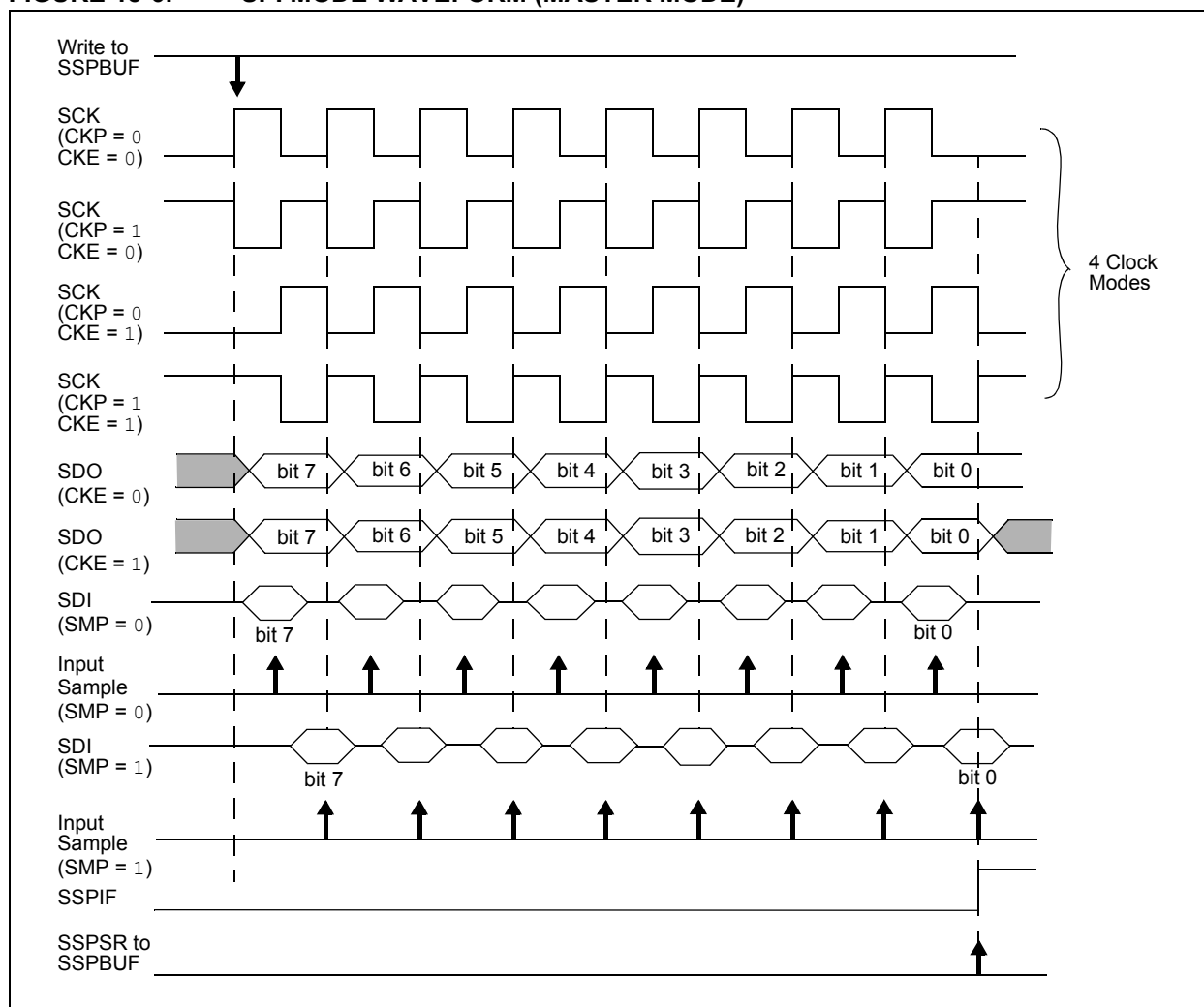
FIGURE 18-6: SPI MODE WAVEFORM (MASTER MODE)
