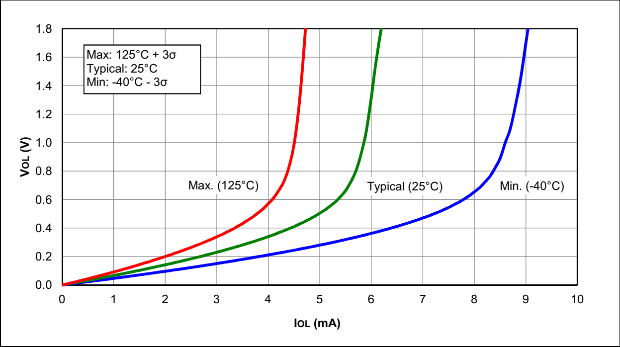
FIGURE 22-17: V_{OL} vs. I_{OL} OVER TEMPERATURE, V_{DD} = 1.8V
