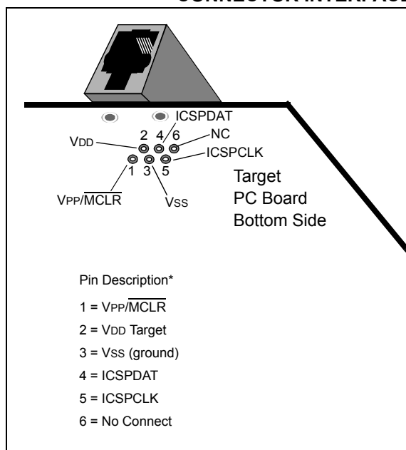
FIGURE 19-1: ICD RJ-11 STYLE CONNECTOR INTERFACE
