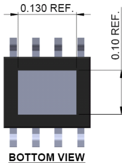
EXPOSED PADDLE
