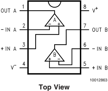
8-Pin SO/MSOP
