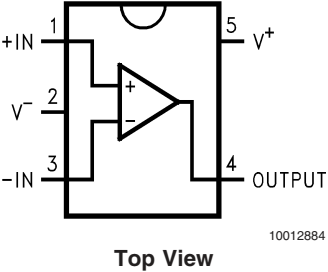
5-Pin SC70-5/SOT23-5
