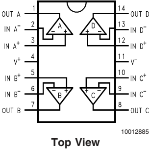
14-Pin SO/TSSOP
