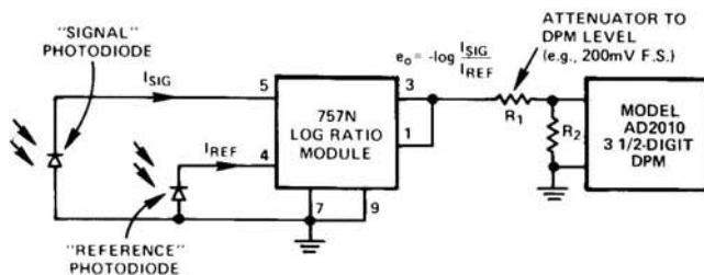
Figure 6. Model 757N Applied to Absorbance Measurements
