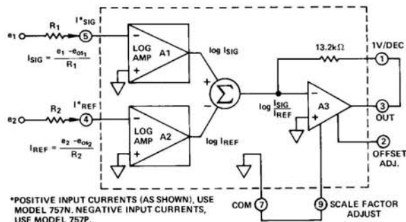
Figure 1. Functional Block Diagram of Model 757
