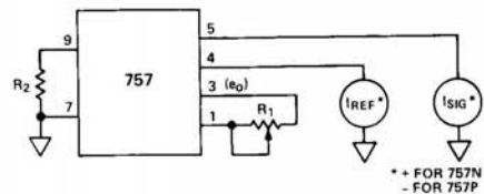
Figure 2. Scale Factor Adjustment
