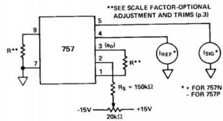
Figure 3. Output Voltage Offset Adjustments
