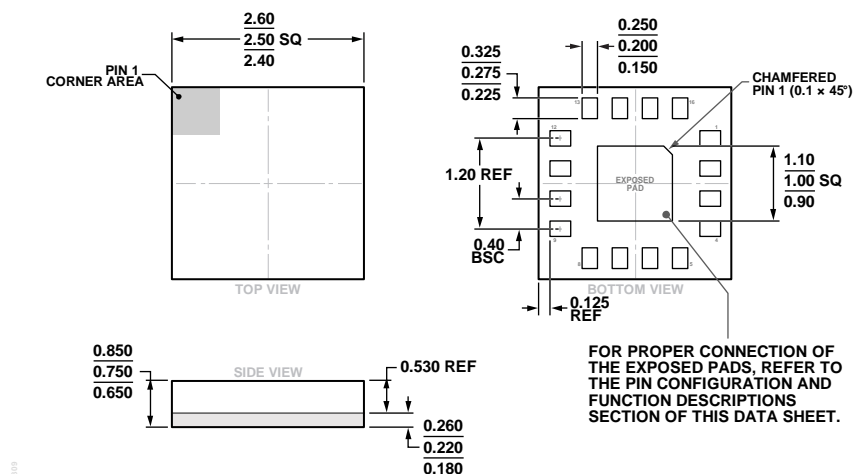
Figure 34. 16-Terminal Land Grid Array [LGA] 2.5 mm x 2.5 mm Body and 0.75 mm Package Height (CC-16-6) Dimensions shown in millimeters
