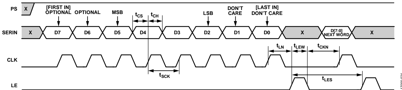
Figure 24. Serial Control Timing Diagram
