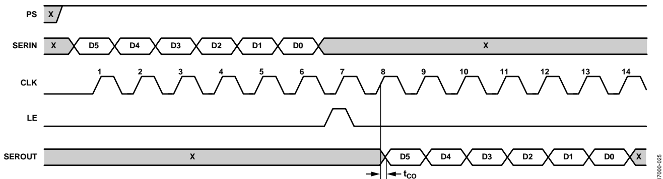
Figure 25. Serial Output Timing Diagram
