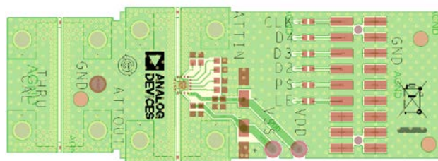
Figure 29. Evaluation Board Layout, Top View
