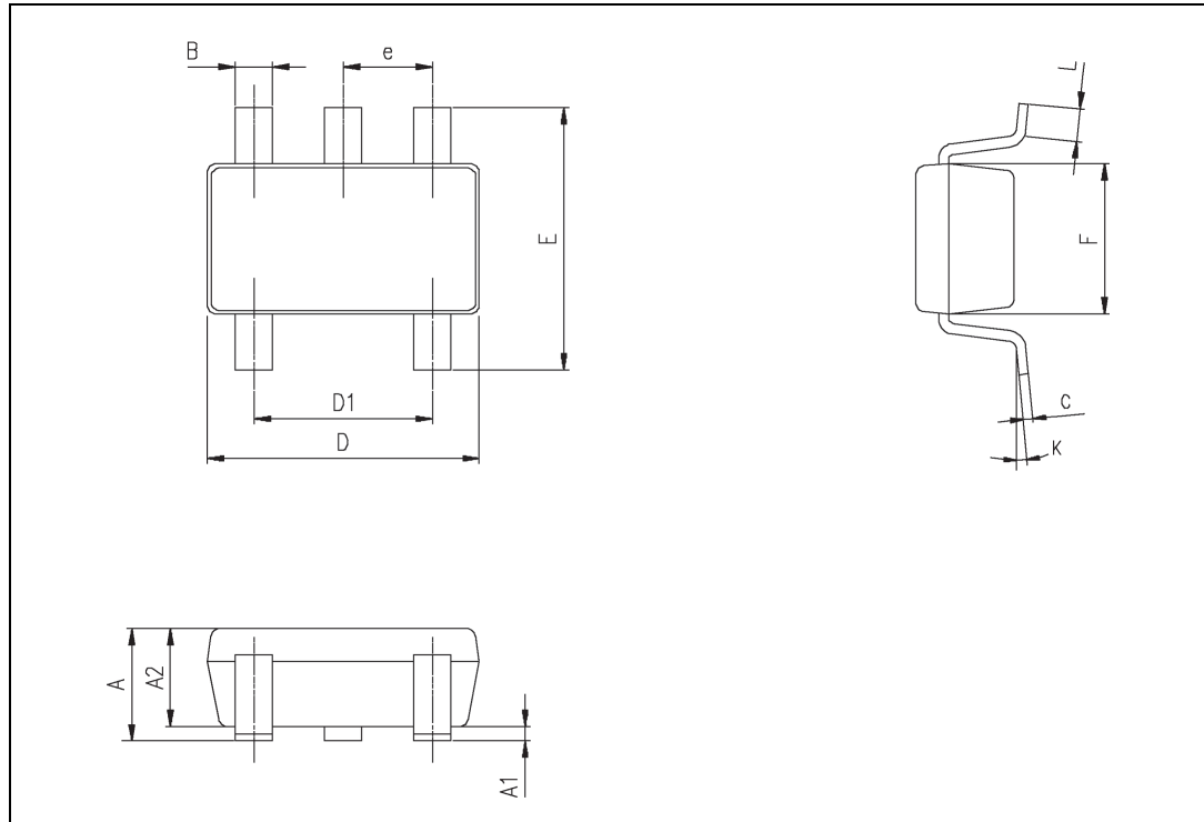
Figure 26. SOT23-5 package mechanical drawing
