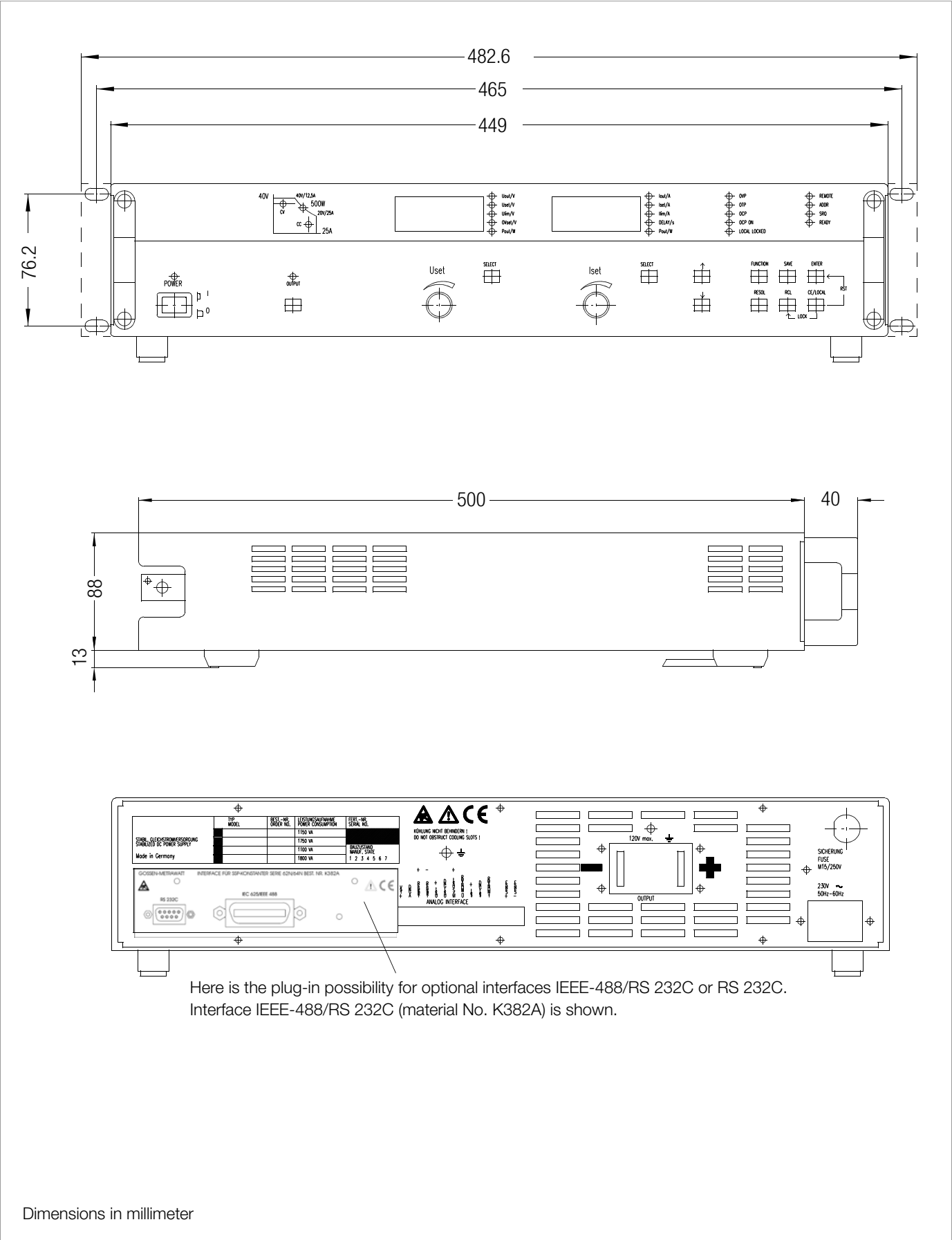
Dimensional Drawing
