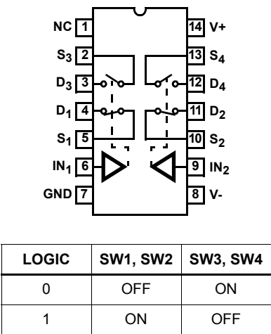
HI-303 (PDIP, Cerdip, SOIC) TOP VIEW
