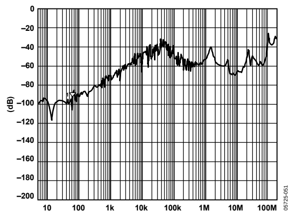
Figure 47. ADR121/ADR125/ADR127 PSRR
