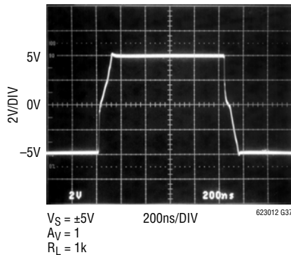
Large-Signal Response
