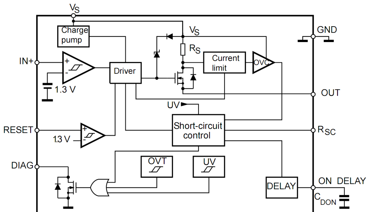
Figure 1. Block diagram
