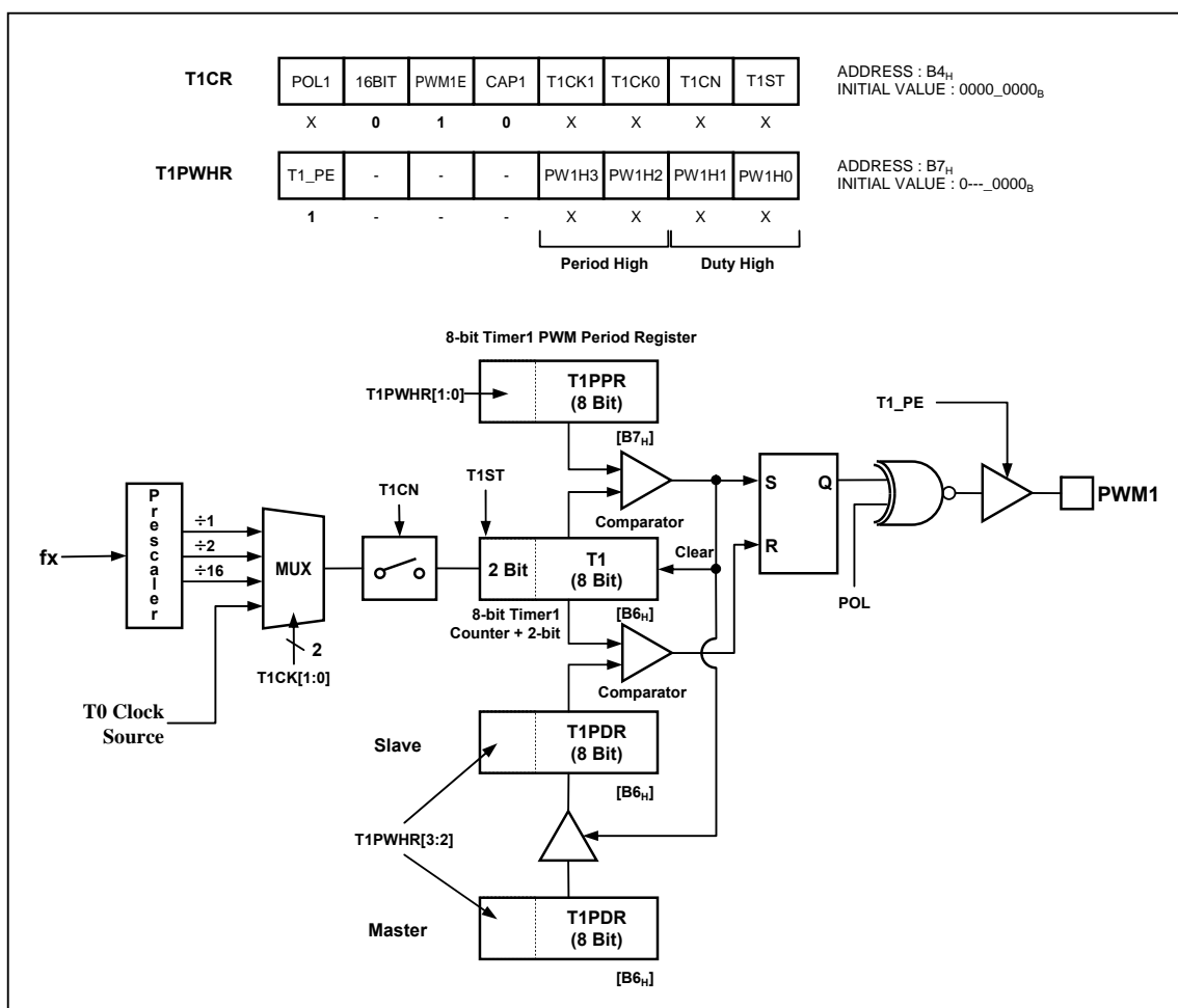
Figure 11-14 PWM Mode
