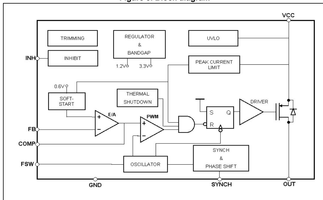
Figure 3. Block diagram
