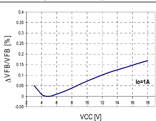
Figure 29. Line regulation
