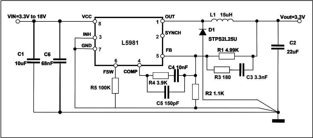
Figure 18. Demonstration board application circuit
