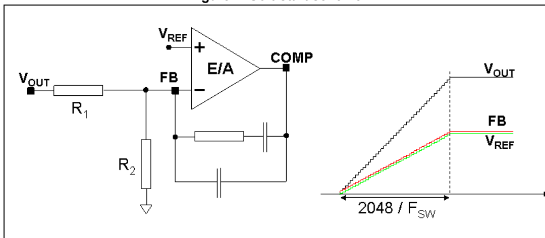
Figure 7. Soft-start scheme
