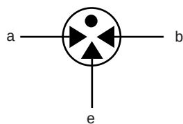
3 ELECTRODE GDT
