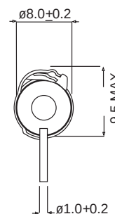
2) 4.4 Leg Pitch = R SL1024A xxxR
