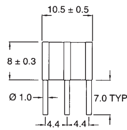
2) 4.4 Leg Pitch = R SL1024A xxxR
