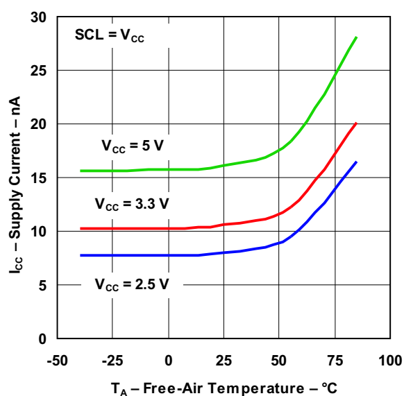
STANDBY SUPPLY CURRENT VS TEMPERATURE
