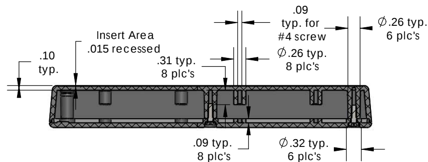
Notes: Enclosure weight .34 lbs /154 gm 1) Enclosure meets or exceeds IP40 and NEMA 1 2) Circuit Board drawings can be download at: http://www.serpac.com/Accessories/CircuitBoard/drawings/370-470.pdf 3) All components are RoHS Compliant.
