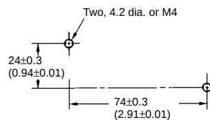
Mounting Holes
