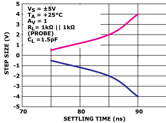
FIGURE 28. STEP SIZE vs SETTLE TIME
