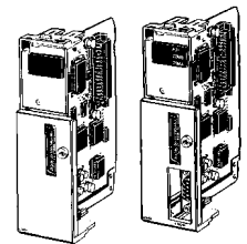
Communications Board C200HW-COM01 C200HW-COM04-E (w/RS-232C port)
