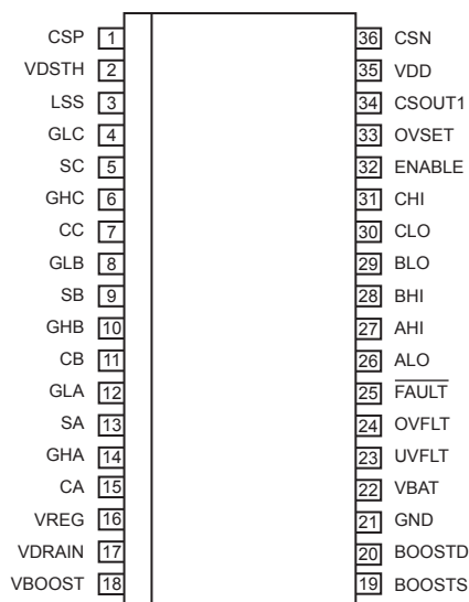
Pin-out Diagram
