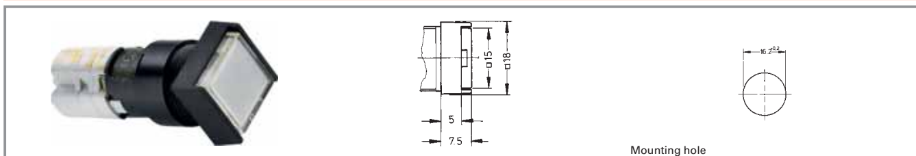
Mounting hole
