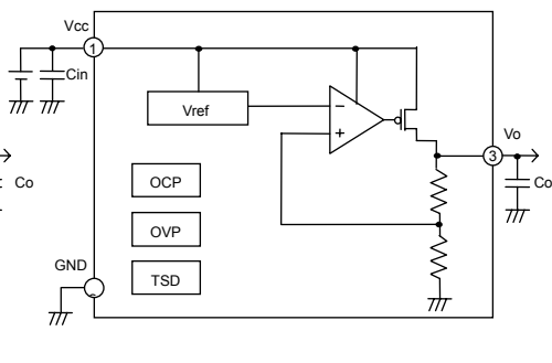
Fig.15 TO220FP-3
