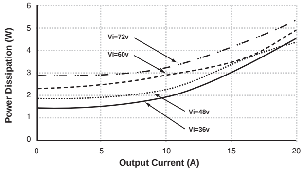
Power Dissipation vs. Output Current for 1.5V/20A PKM4318PIOA
