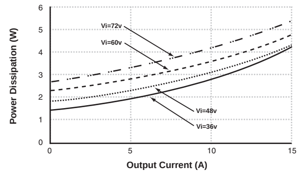
Power Dissipation vs. Output Current for 2.5V/15A PKM4319PI
