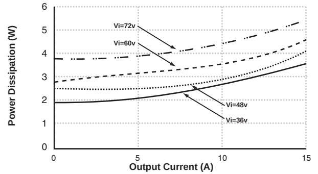
Power Dissipation vs. Output Current for 1.8V/15A PKM4218PI
