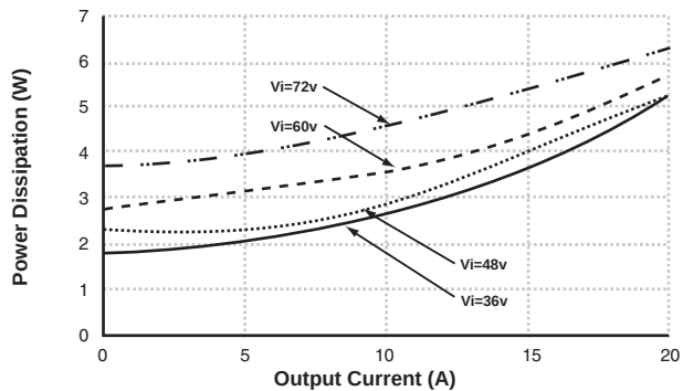
Power Dissipation vs. Output Current for 1.8V/20A PKM4318PI
