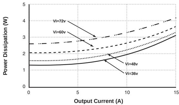
Power Dissipation vs. Output Current for 1.5V/15A PKM4218PIOA
