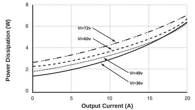
Power Dissipation vs. Output Current for 2.5V/20A PKM4519PI
