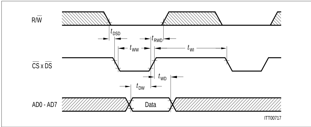
Figure 40 \mu P Write Cycle
