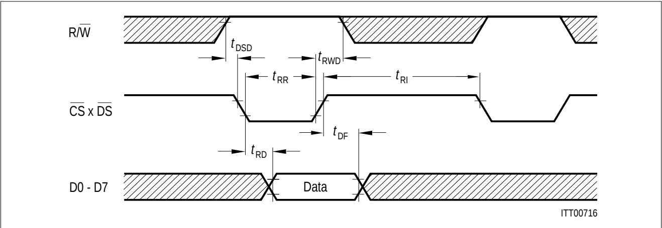
Figure 39 \mu P Read Cycle
