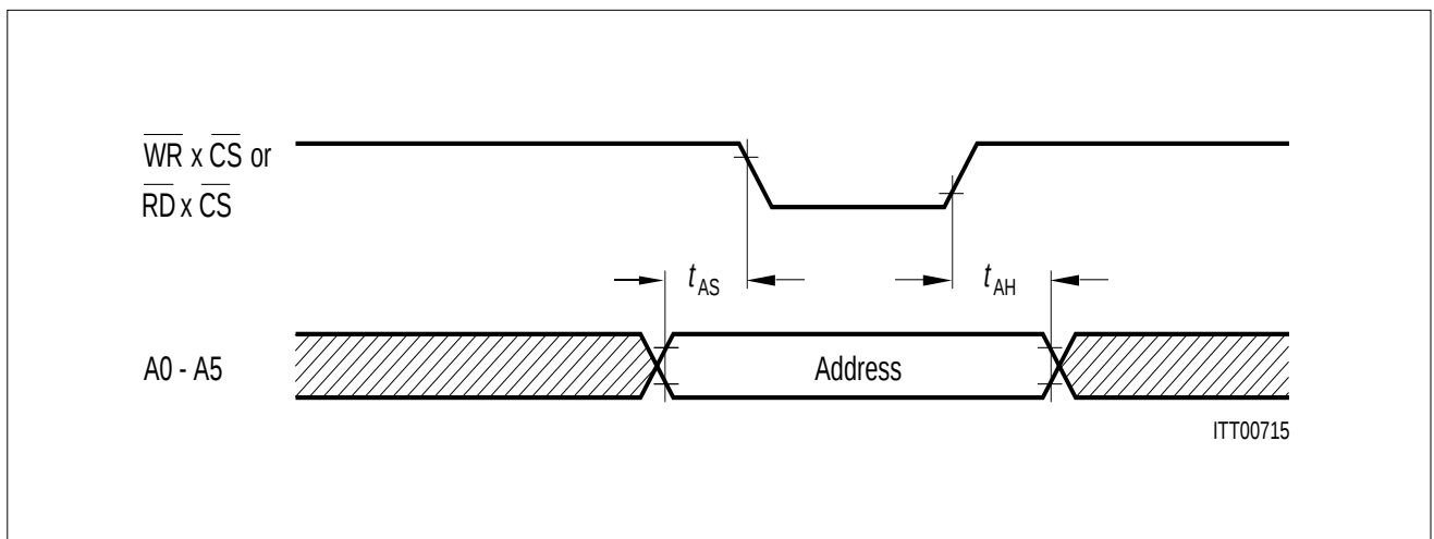
Figure 38 Non-Multiplexed Address Timing
