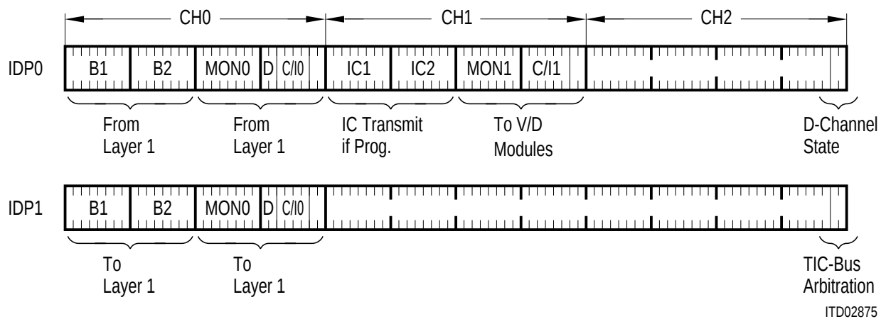
(a) ICC Master Mode (IDC = 0)
