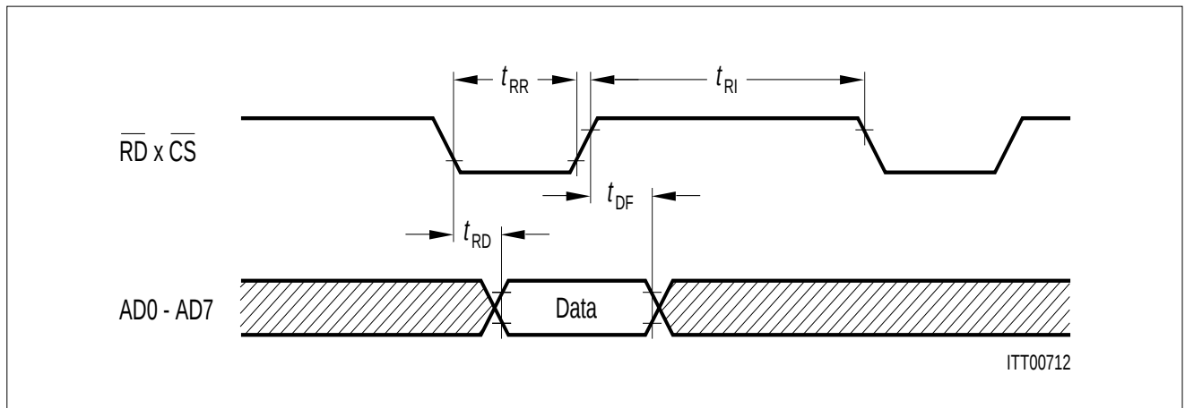
Figure 35 \mu P Write Cycle
