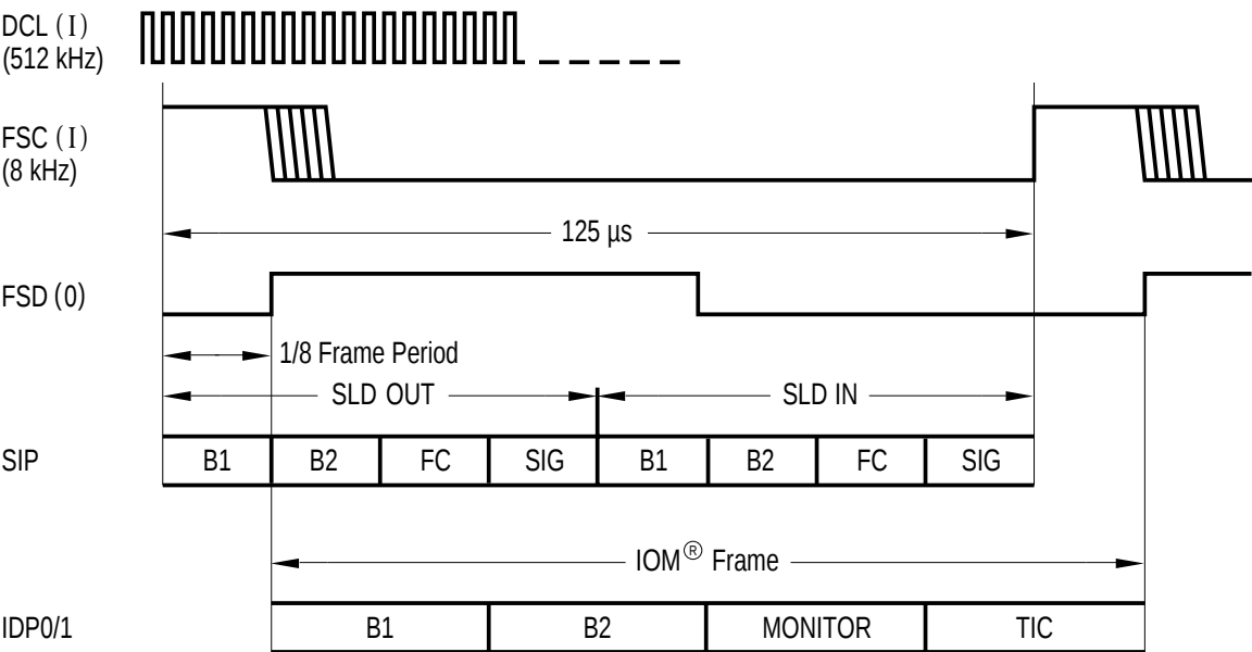
(b) Timing Mode 1
