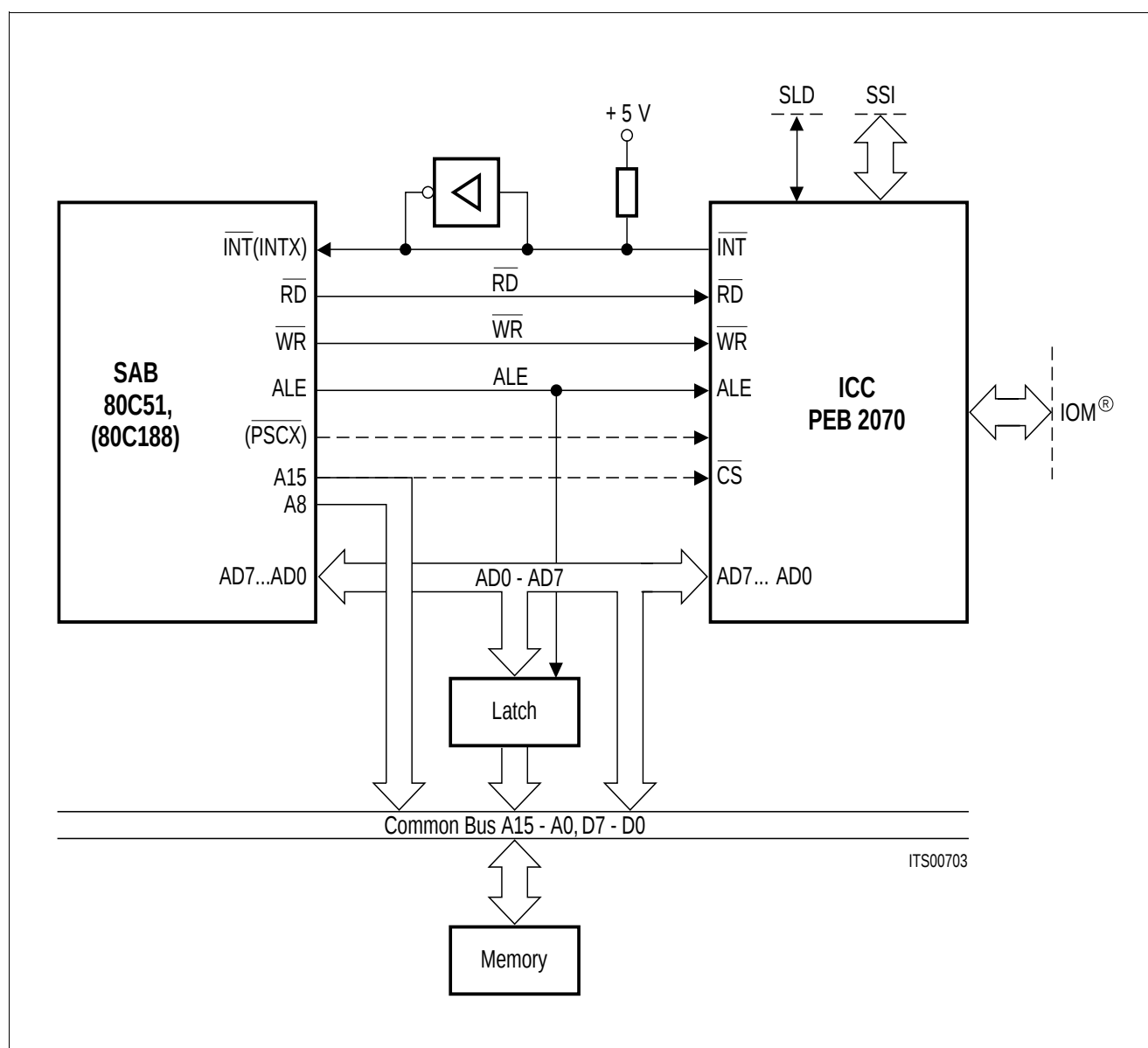
Figure 5 Example of ICC Microcontroller Environment
