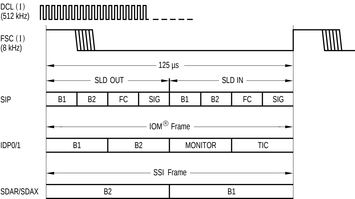
(a) Timing Mode 0
