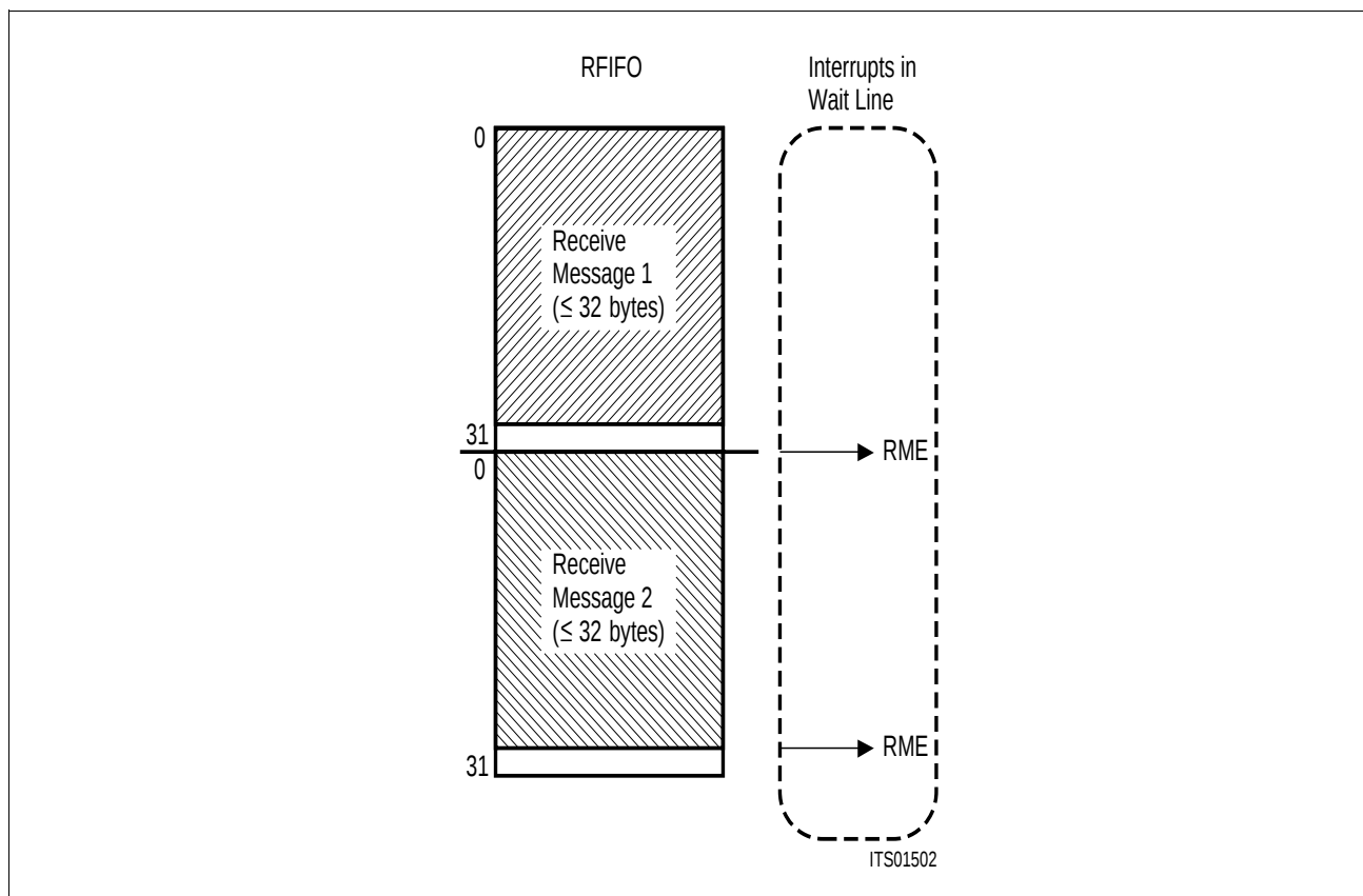
Figure 14 Contents of RFIFO (short message)
