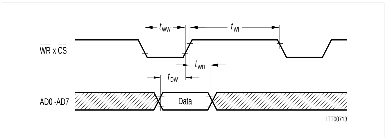
Figure 36 \mu P Write Cycle
