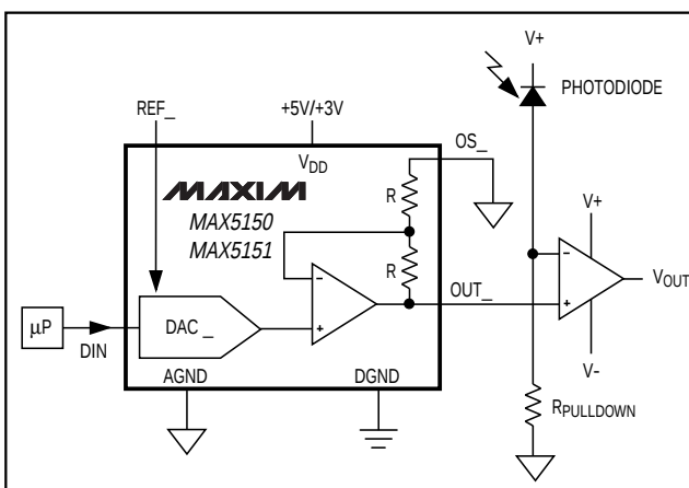
Figure 13. Digital Calibration
