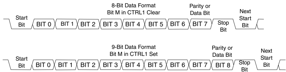
Figure 31-2. SCI Data Frame Formats
