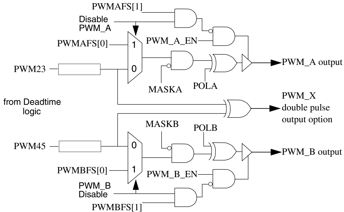
Figure 27-24. Output Logic
