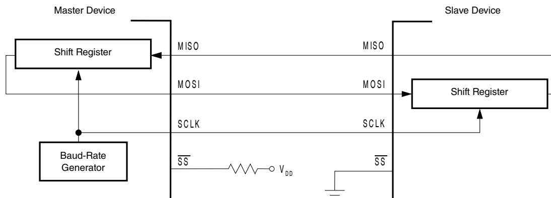
Figure 32-2. Full-Duplex Master-Slave Connections
