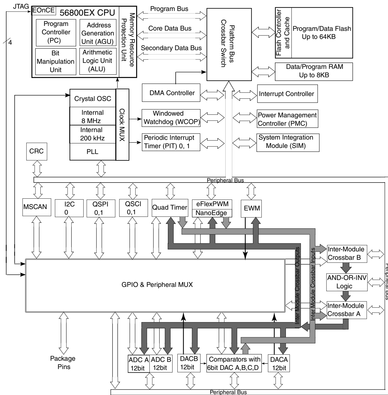
Figure 2-1. Block Diagram
