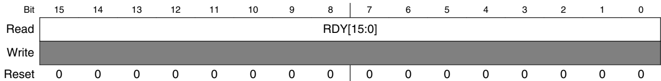
ADC_RDY field descriptions
