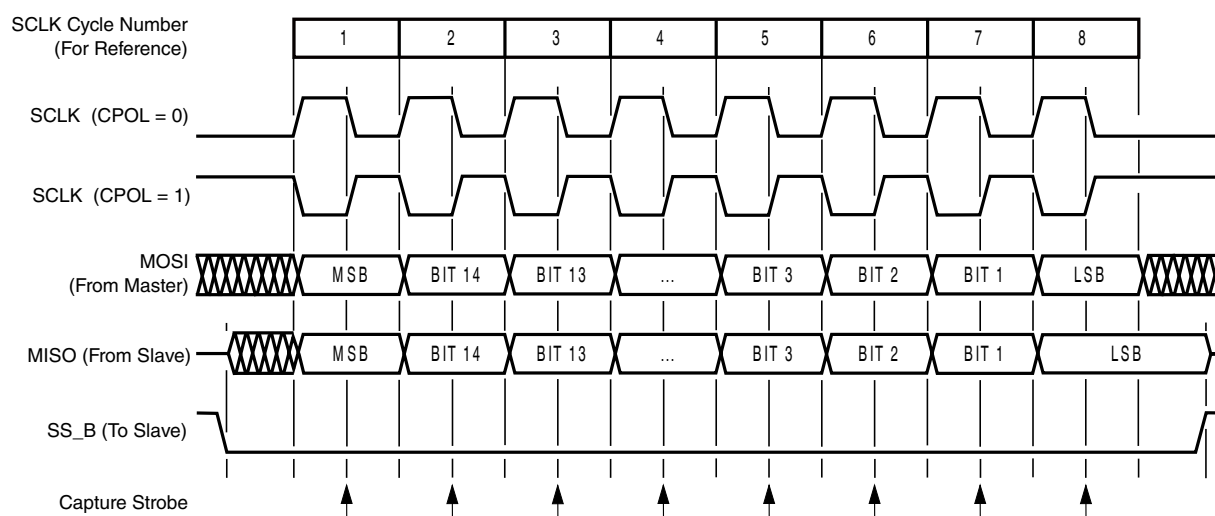
Figure 32-7. Transaction Format ( \text{CPHA} = 1 )
