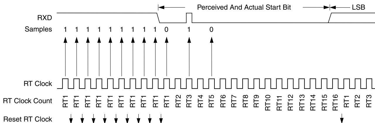
Figure 31-9. Start Bit Search Example 4
