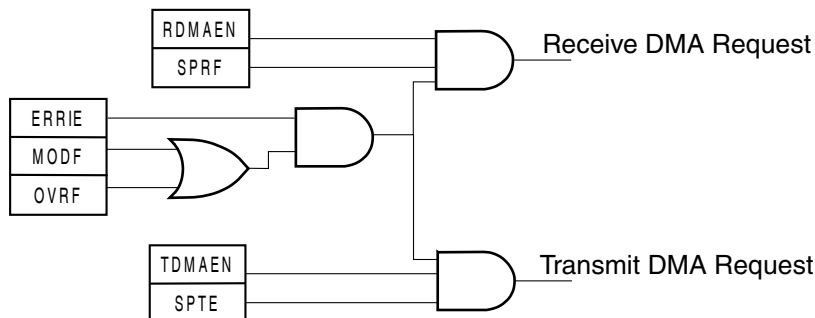
Figure 32-3. SPI DMA Request Generation
