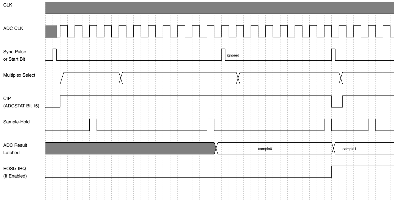
Figure 24-11. ADC Timing
