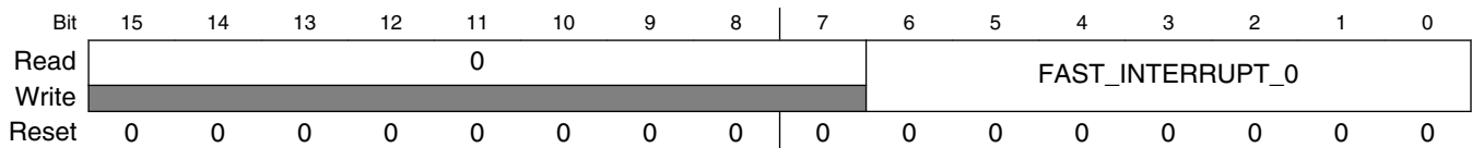
INTC_FIM0 field descriptions
