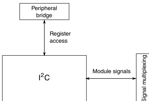
Figure 3-22. I2C configuration
