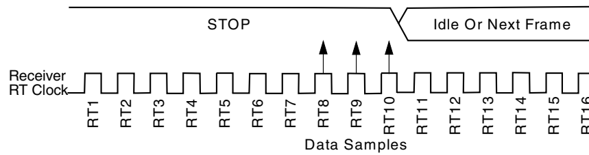
Figure 31-13. Fast Data
