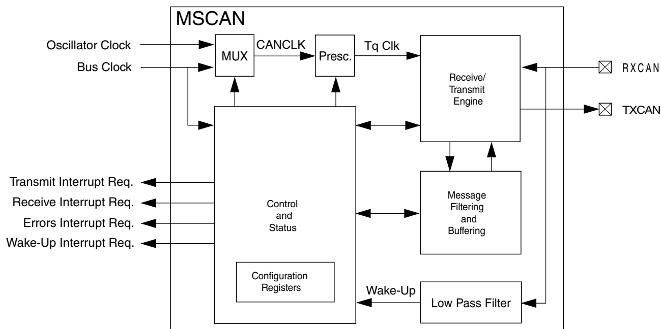
Figure 30-1. MSCAN Block Diagram
