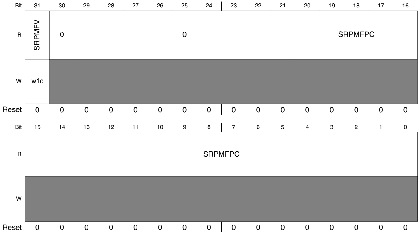
MCM_SRPMP field descriptions
