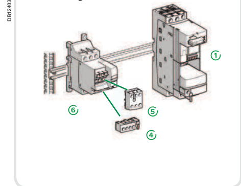
Side mounting
