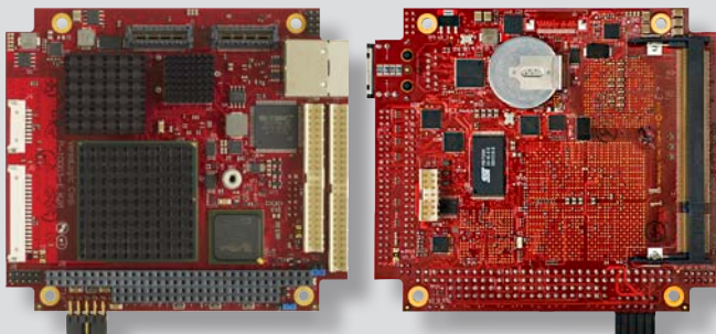
VL-EPMs-21g (Top)
