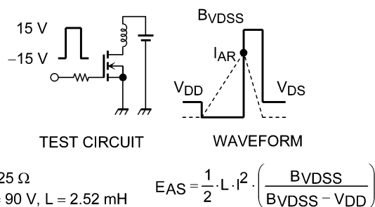
Fig. 8.16 Test Circuit/Waveform
