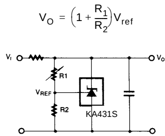
Figure 13. Shunt Regulator
