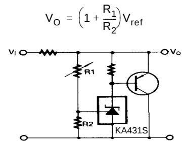
Figure 15. High Current Shunt Regulator
