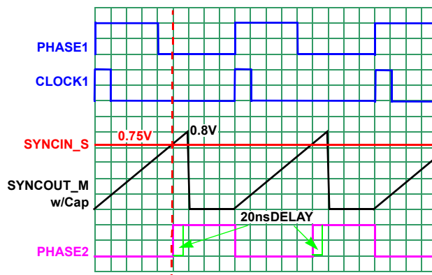
FIGURE 36. SYNCHRONIZATION WAVEFORMS
