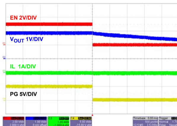
FIGURE 26. SOFT-DISCHARGE SHUTDOWN
