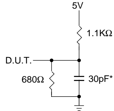
Figure A. Output Load
