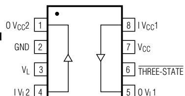
SOT23-8 TOP VIEW
