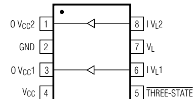
TDFN-8 (3mm x 3mm) TOP VIEW
